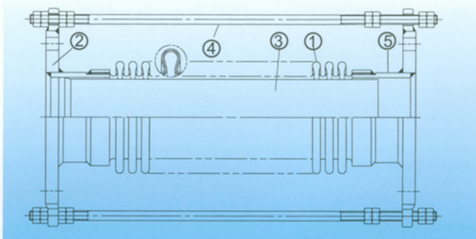
有內筒及設限螺桿 With internal sleeve and Tie Rod.
